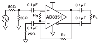
Figure 5. Single-Ended Application
